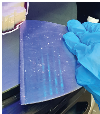
Figure 5: Removing the part with a scraper
